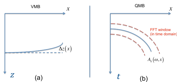
Figure 2 Q-RMO measures depth residuals for velocity updates (a) and spectral ratios for Q updates (b).
